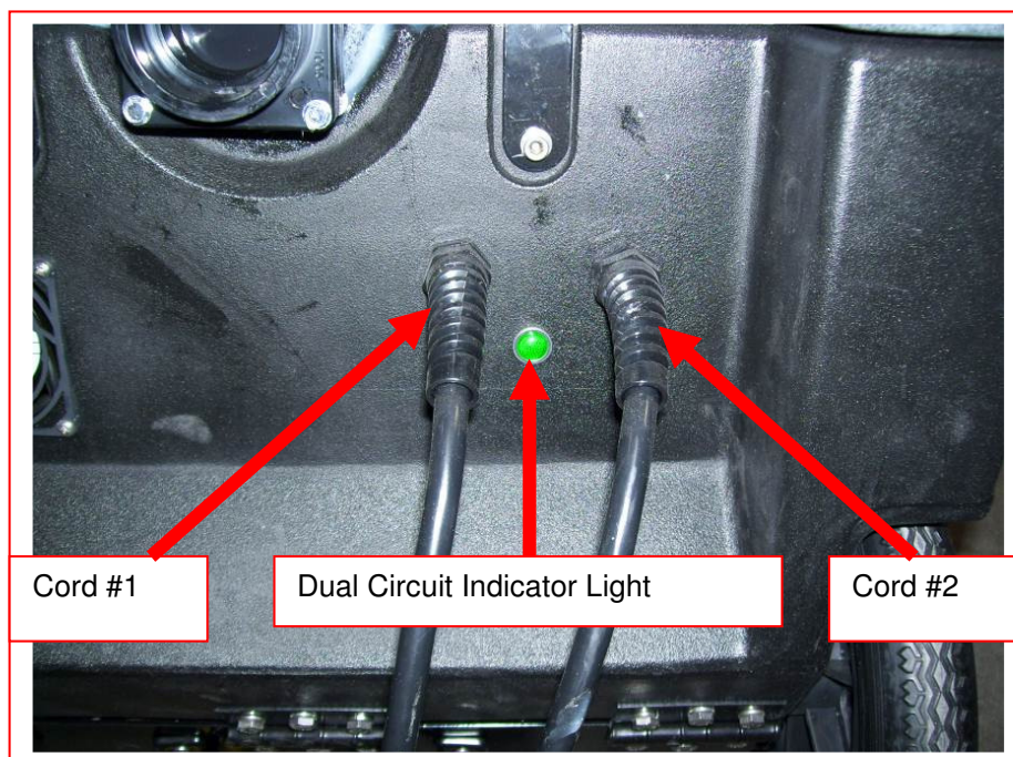
Power Cord – 1696-6412 25' – 10 gauge M-F Plugs
