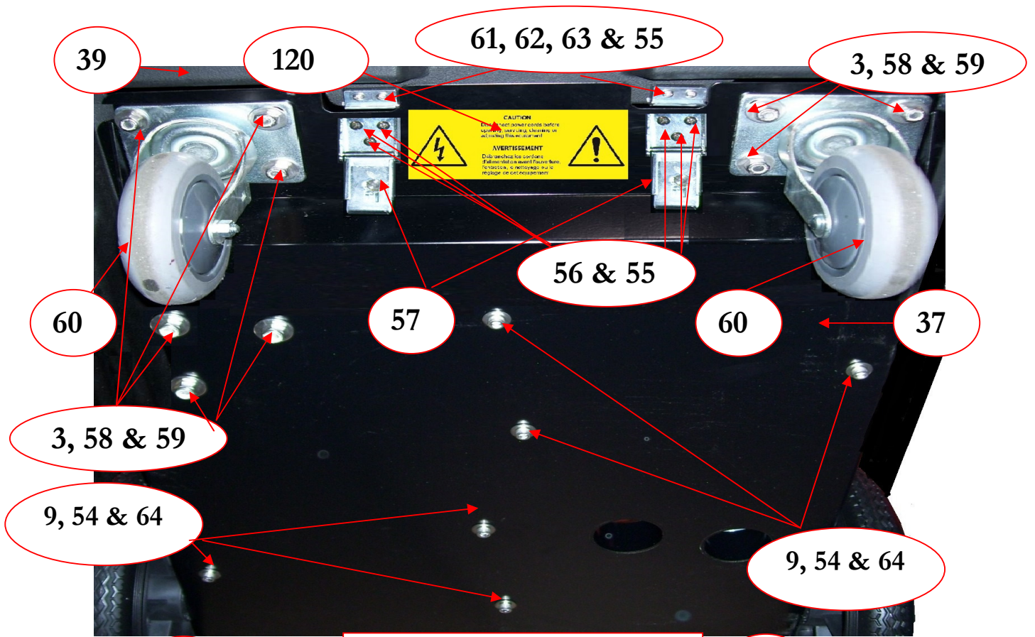
BOTTOM VIEW OF BASE
